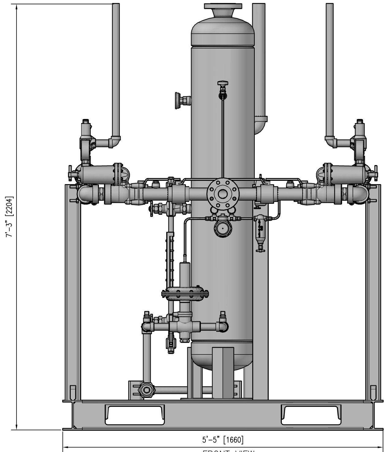
FRONT VIEW
